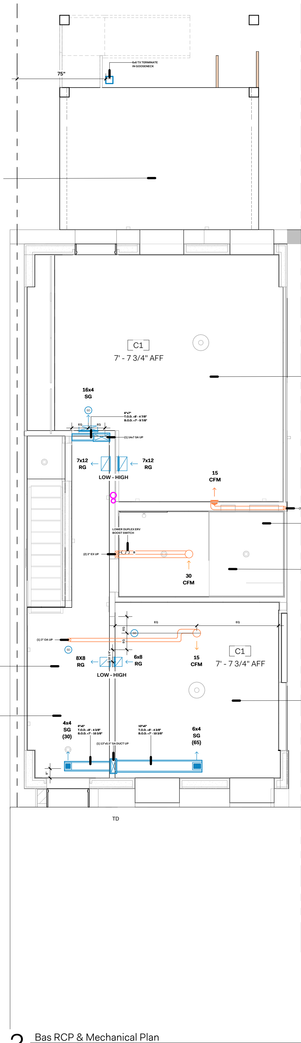
2 Bas RCP & Mechanical Plan 1/4" = 1'-0"
